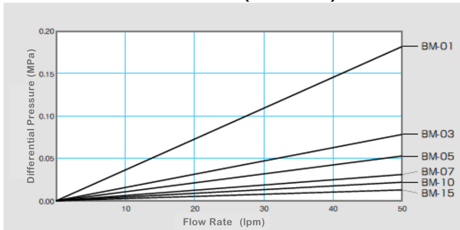
Flow Rate-Differential Pressure (Per 250mm)
