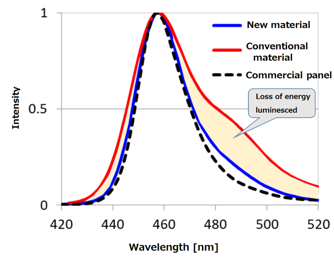
Fig. 1 Luminescence Spectrum
